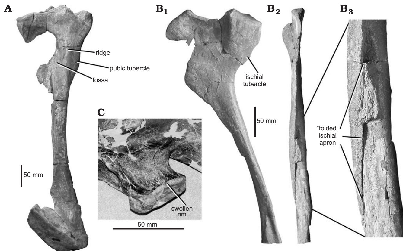
Fig. 3. Autapomorphies of tyrannosauroids Juratyrant langhami Benson, 2008, Kimmeridge Clay, Dorset England, Late Jurassic (early Tithonian) (A, B) and Stokesosaurus clevelandi Madsen, 1974, Morrison Formation, Utah, USA, Late Jurassic (early Tithonian) (C). A. Right pubis (OUMNH J.3311-22) in lateral view, with the autapomorphic lateral fossa denoted. B. Left ischium (OUMNH J.3311-25) in lateral (B 1 ) and anterior (B 2 ) views, with an inset close up (2.5× magnification) of the autapomorphic folded proximal region of the ischial apron (B 3 ). The autapomorphic convex ischial tubercle is also denoted. C. Pubic peduncle of the left ilium (UMNH 2938) in medial view, with the autapomorphic swollen rim indicated.
