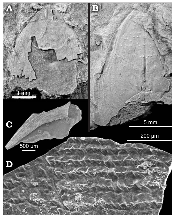
Fig. 3. Linguloid Leontietta sp. from the Early Ordovician Fenxiang Formation of Hubei Province, China. A. Incomplete ventral interior showing pseudointerarea and pedicle groove (ZPAL Bp 70/1). B. Incomplete dorsal internal mould showing median ridge (ZPAL Bp 70/2). C. Fragment of ventral valve showing left pseudointerarea and partly preserved pedicle groove (ZPAL Bp 70/3). D. External surface ornament (ZPAL Bp 70/4). C, D, SEM micrographs.
