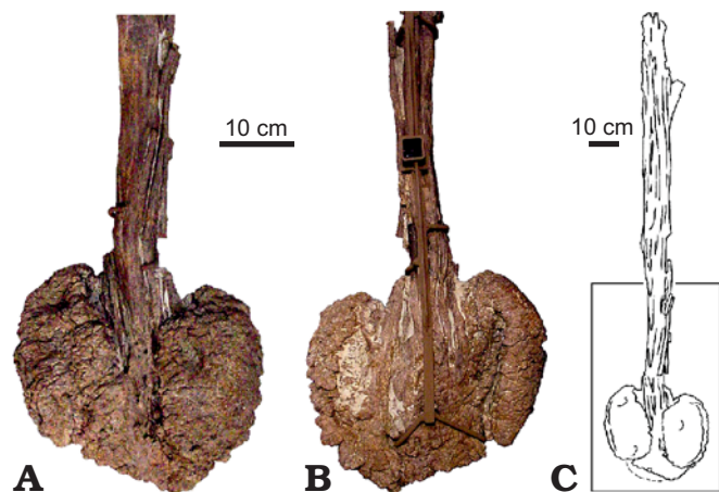
Fig. 8. Well preserved tail club of ankylosaurid dinosaur TMP 2001.42.19, referred specimen of Oohkotokia horneri sp. et gen. nov. from the late Campanian Two Medicine Formation of Montana, in dorsal ( A ) and ventral ( B ) views. The complete tail club ( C ); rectangle shows area of photos.
