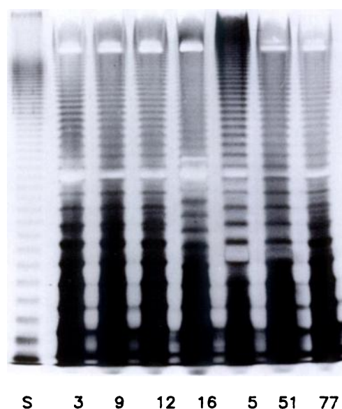
FIGURE 3. SDS-PAGE of proteinase K treated bacterial sonicates stained to visualize structural lipopolysaccharide characteristics as discussed by Hitchcock and Brown (1983). The E. ictaluri isolates 3, 9, 12, 51, and 77 were derived from ictalurid hosts and represent the typical profile observed for most of the 32 isolates examined. Isolate 5 from a catfish and isolate 16 from green knife fish show some of the minor structural variations observed in the electrophoretic migration of the repeating subunits of the O-antigen side chain. Reference LPS from Salmonella typhimurium (S; Sigma Chemical Co., St. Louis, Missouri 63178, USA) was run as a standard control.
