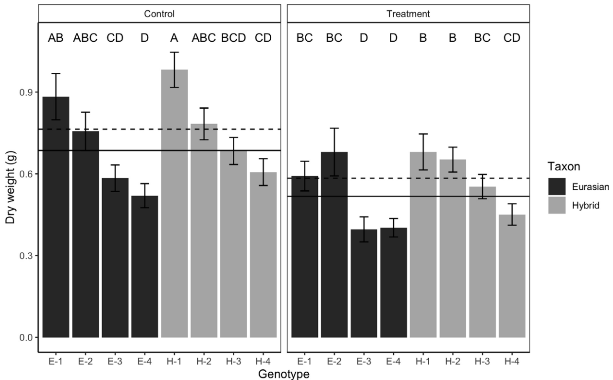
Figure 1. Average dry weight (g ± SE) values for eight genotypes of invasive Myriophyllum : four Myriophyllum spicatum (black bars) and four Myriophyllum spicatum × sibiricum (gray bars). Each of the genotypes is represented by a letter+number combination for figure clarity. The letter indicates the taxon associated with each genotype: E, Eurasian watermilfoil ( Myriophyllum spicatum ); H, hybrid watermilfoil ( Myriophyllum spicatum × sibiricum ). The number indicates its within-taxon ranking in mean growth rate. The dashed line denotes mean dry weight for M. spicatum × sibiricum hybrids in each treatment type, and the solid line denotes mean dry weight for pure M. spicatum in each treatment type. Different letters represent significant differences between genotypes across both control and treatment.
