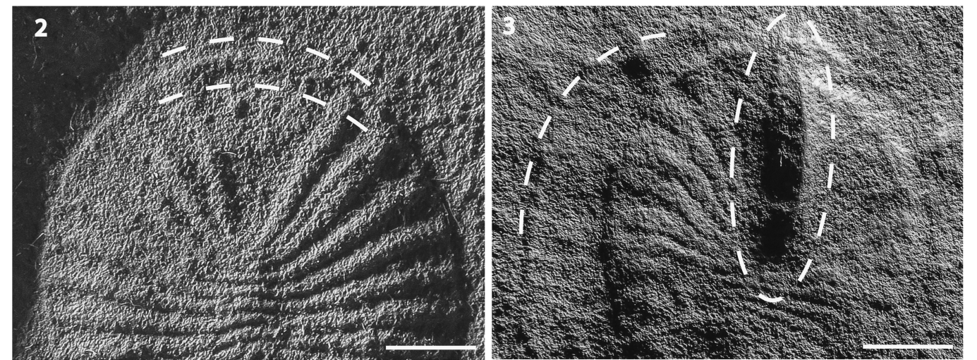
Figure 2. (1) Descriptive labels for Dickinsonia costata features: 1 = terminal A-end unit, 2 = body unit, 3 = position of shrinkage rim, 4 = position of A-end lip, 5 = generalized position of A-end protuberance. (2) Detail of A-end lip feature, visible as a narrow, raised rim on the peripheral margin of the terminal A-end unit, SAMP34228. (3) Detail of shrinkage rim feature as an uneven margin exterior to the body fossil, and the A-end protuberance as a high relief, elongate structure involving the terminal A-end unit and several A-end units, SAMP34232. The surface visible is assumed to be the upper surface. Scale bars = 3mm.
