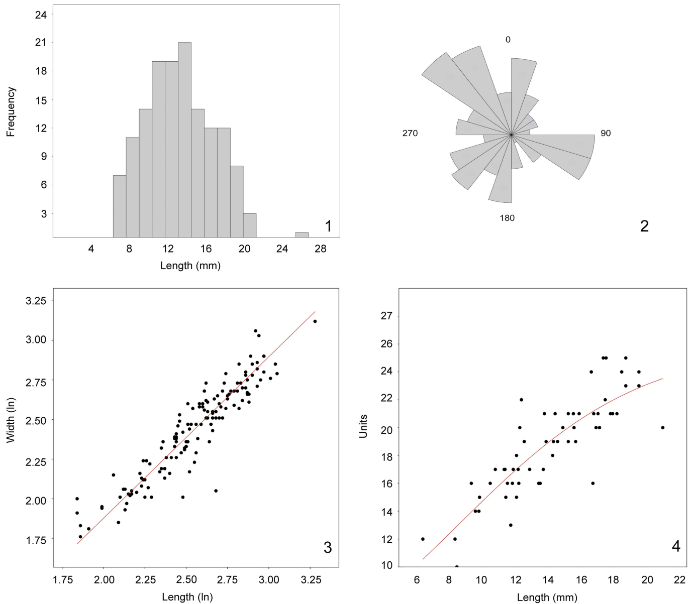
Figure 3. Analyses of Dickinsonia costata population. (1) Histogram showing size distribution of population (N=140); (2) rose diagram showing axial alignment of specimens (N=118); the ‘0’ is an arbitrary reference and denotes the top of the “Crisp Wall” frame; (3) graph depicting the relationship between (ln) length and (ln) width of specimens (N=140); (4) logistic graph depicting the relationship between specimen length and number of observable units (N=58).
