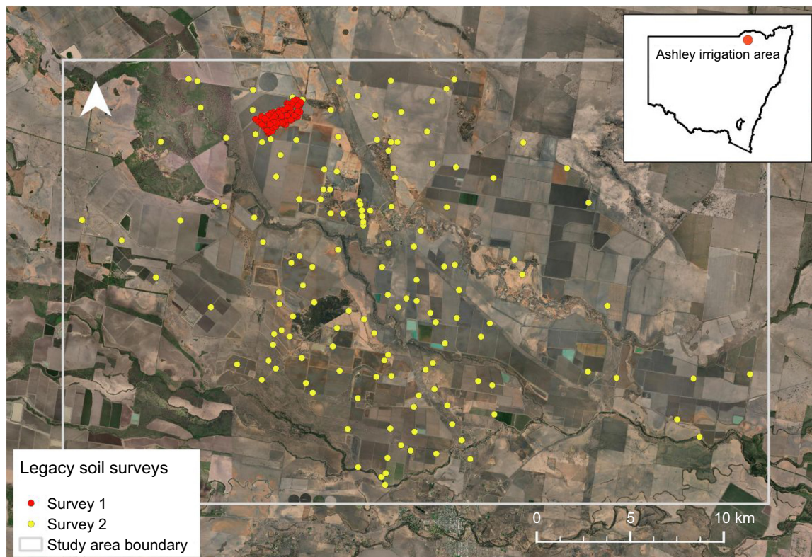
Fig. 1. Location of the Ashley Irrigation Area relative to New South Wales, and the location of legacy soil surveys across the Ashley Irrigation Area.
