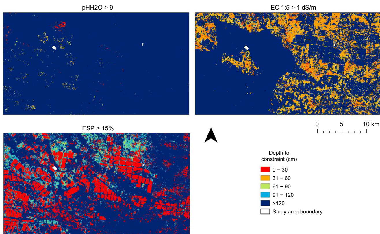
Fig. 3. The depth-to three constraint thresholds: \text{pH}_{\text{H}_2\text{O}} > 9 , \text{EC}_{1:5} > 1 dS/m, \text{ESP} > 15\% .
