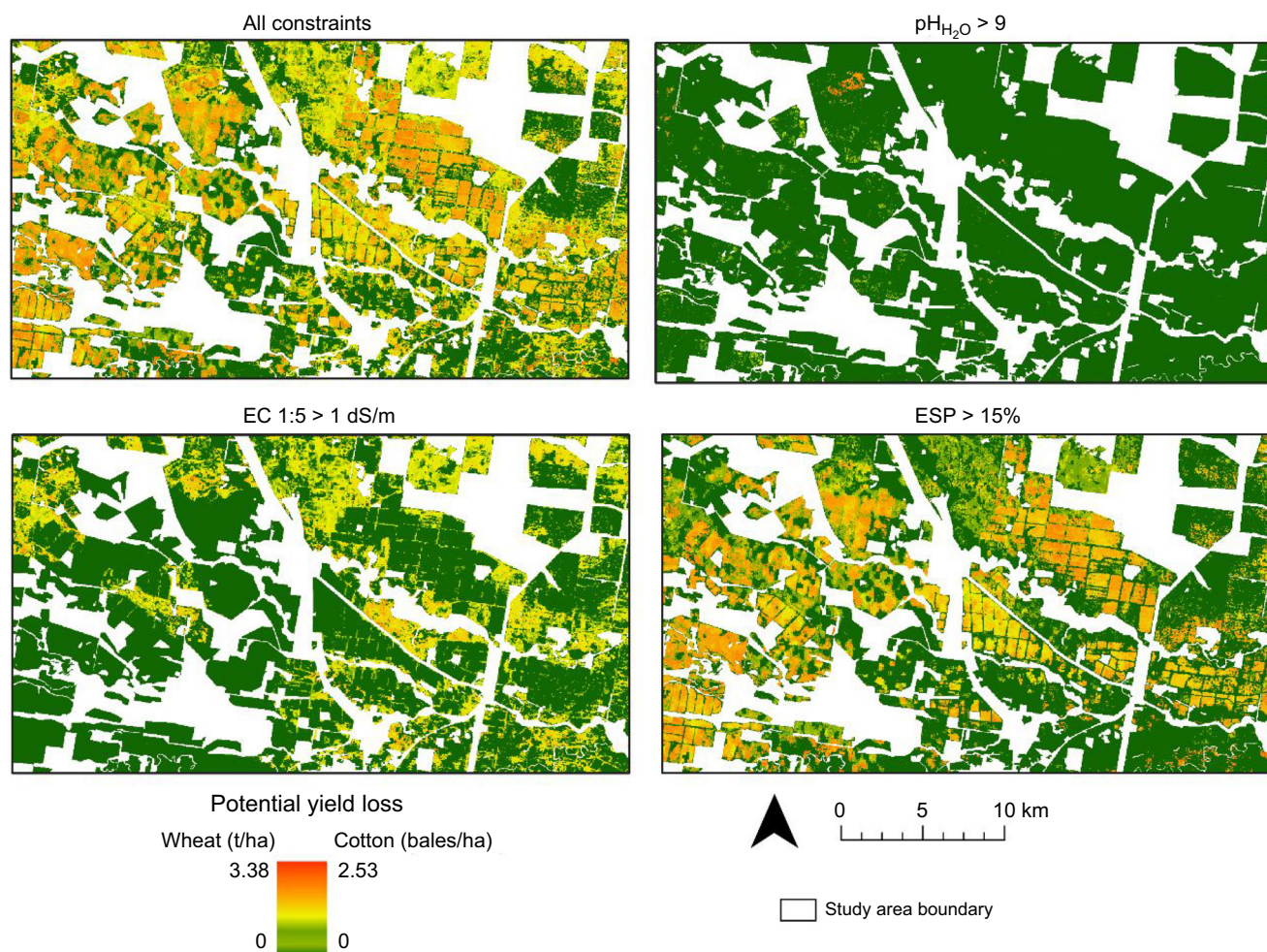
Fig. 5. Potential yield loss due to all constraints, and due to the presence of individual constraints \text{pH} > 9 , \text{EC}_{1:5} > 1 dS/m, and \text{ESP} > 15\% for cotton and wheat on arable land.
