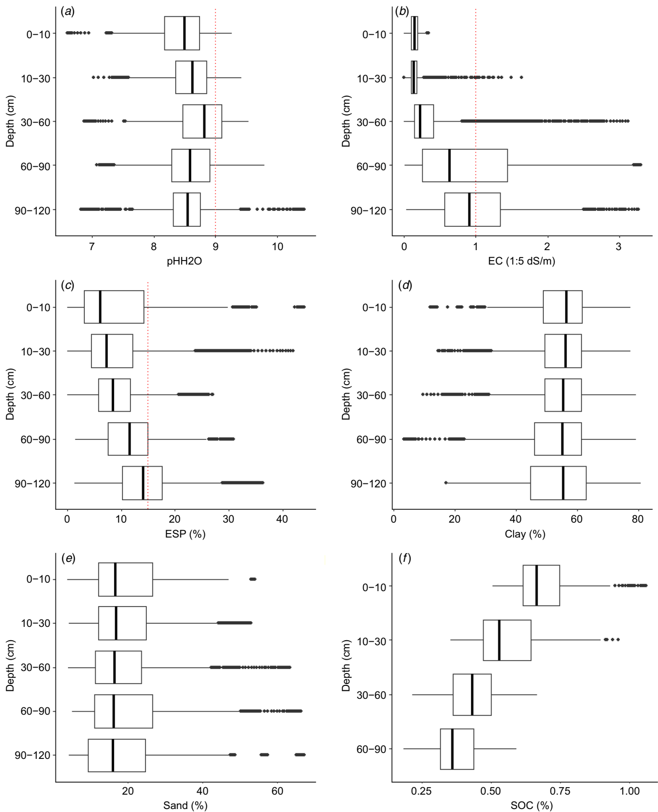
Fig. 2. Boxplots of soil pH H 2 O (a), EC 1:5 (b), ESP (c), clay (d), sand (e), and SOC (f) attribute values with depth. Median values represented by solid black lines inside boxes, and the dashed vertical red lines indicate the threshold values deemed to be constraining to crop growth for pH, EC, and ESP (pH H 2 O 9, EC 1:5 1 dS/m, ESP 15%). No data for SOC were available for a depth > 90 cm.
