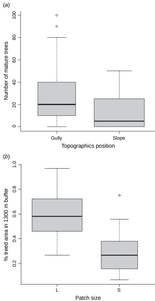
Fig. A2. Relationship between (a) topographic position and density of large trees (DBH > 60 cm) at a site; and (b) patch size (large or small) and proportion of tree cover in a 1300-m buffer zone surrounding each site in the study area in north-central Victoria, Australia.
