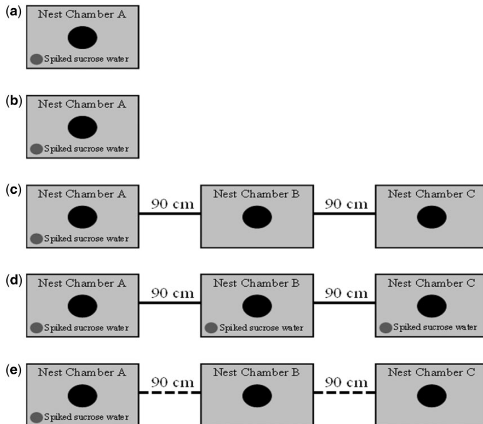
Fig. 1. Laboratory feeding experiment setup (a–e). (a) Feeding experiment 1: monodomous colony, small. (b) Feeding experiment 2: monodomous colony, large. (c) Feeding experiment 3: polydomous colony, localized food source. (d) Feeding experiment 4: polydomous colony, dispersed food source. (e) Feeding experiment 5: polydomous colony, localized food source, delayed foraging. Nest chambers (black, shaded circles) were situated in foraging arenas (27 by 20 by 9.5 cm) connected by wooden bridges.
