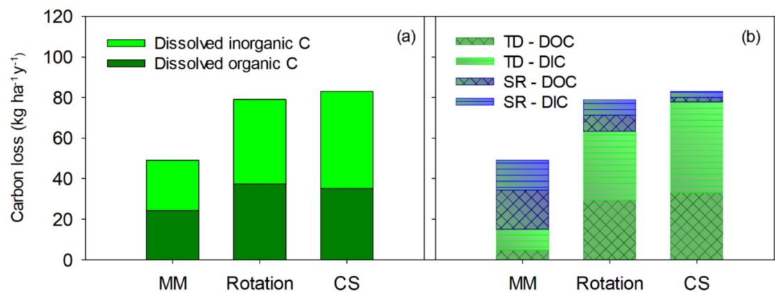
Fig. 6. Partitioning of total carbon loss from monoculture maize (MM), continuous Kentucky blue grass sod (CS), and an alfalfa–maize–oat rotation (Rotation) between: (a) dissolved organic and inorganic carbons; (b) tile drainage and surface runoff.
