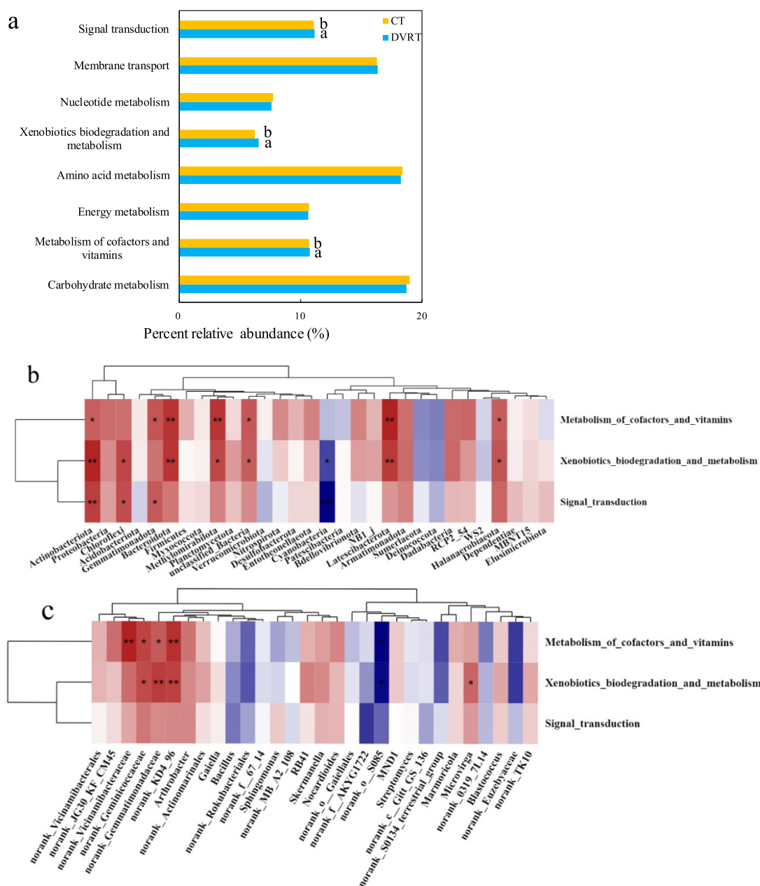
Fig. 5. Tax4Fun prediction of soil bacterial community function under DVRT and CT. (a) Relative major functional groups; different letters indicate statistically significant differences at P < 0.05 as determined by the Student's t test for independent samples. (b) Correlation between bacterial phylum level and predictive function group. (c) Correlation between bacterial genus level and predictive function group. * P < 0.05 , ** P < 0.01 , *** P < 0.001 . DVRT, deep vertical rotary tillage; CT, conventional rotary tillage. [Color online.]
