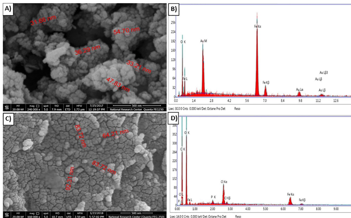
Figure 2. (A) SEM result for nZVI with size between 31 and 60 nm, (B) EDAX analysis of the prepared nZVI, (C) SEM analysis for GT-nZVI with size between 60 and 80 nm, and (D) EDAX analysis of the prepared GT-nZVI. EDX indicates energy-dispersive X-ray; GT-nZVI, green synthesized nano zerovalent iron; nZVI, nano zerovalent iron; SEM, scanning electron microscopy.
