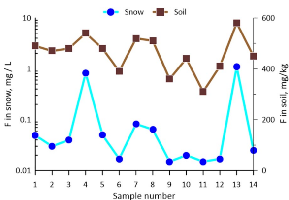
Figure 6. Correlation of F content in snow water ( \text{mg/L} ) and in soil ( \text{mg/kg} ) around the Tayshet aluminum smelter.
