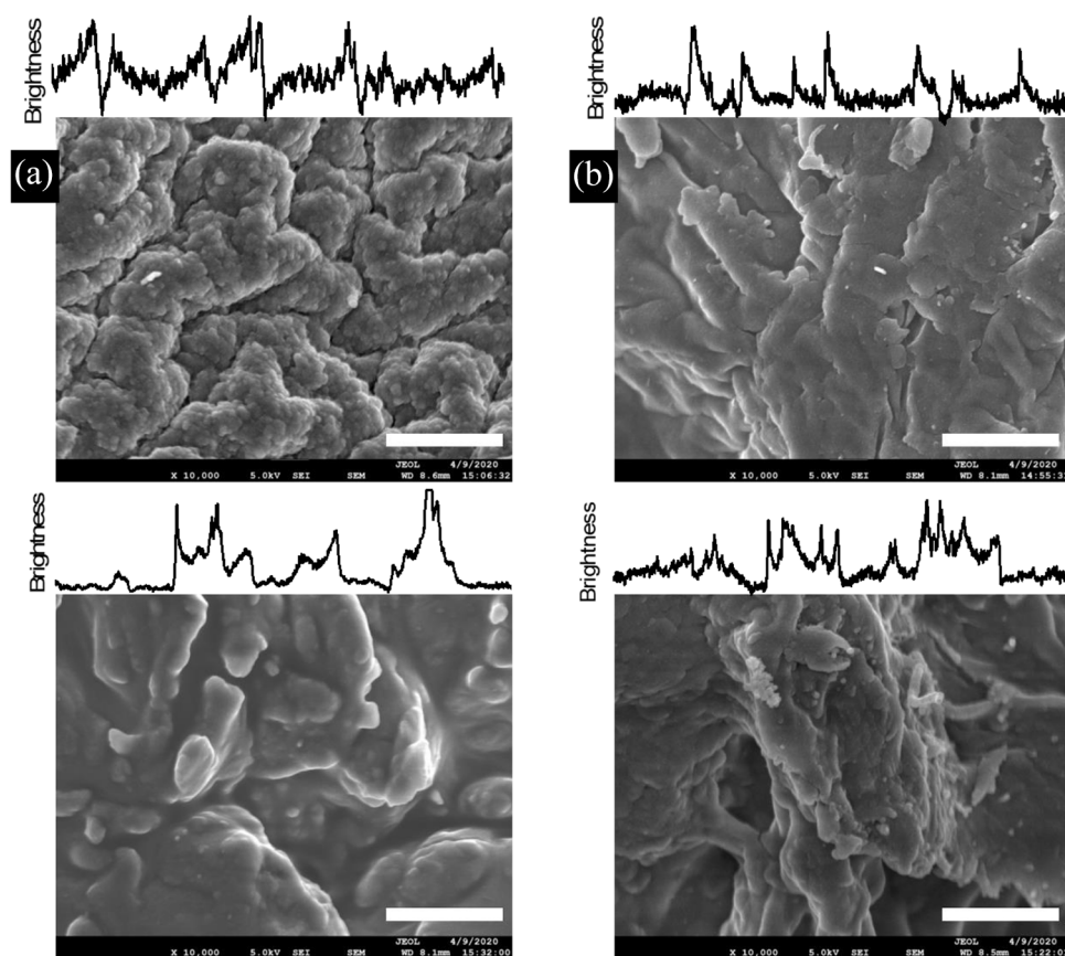
Figure 2. SEM images of (a) BP and (b) DP before (top row) and after AB25 adsorption (bottom row). All images were recorded at the same magnification (10,000 \times ). The scale bars represent 3 \mu\text{m} . The line profiles on top of each image represent horizontal line scans from edge to edge passing through the center of the image.
