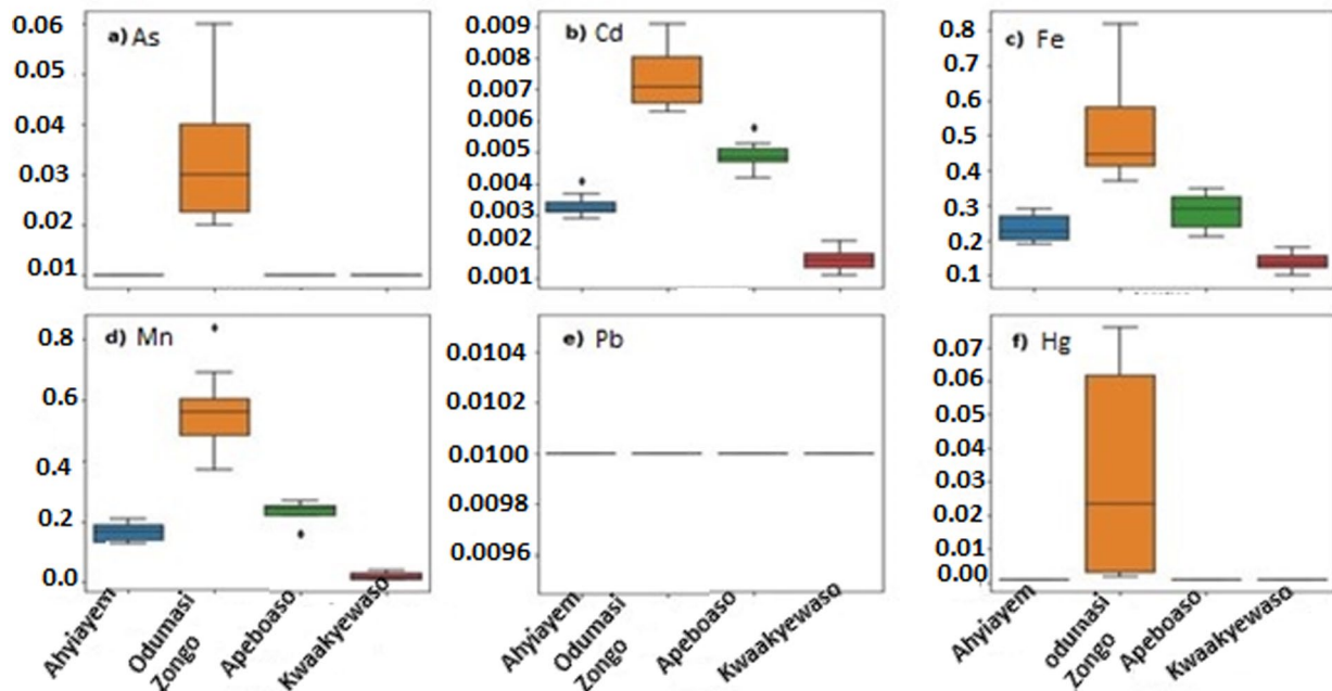
Figure 3. Boxplots of concentrations of: (a) arsenic, (b) cadmium, (c) iron, (d) manganese, (e) lead, and (f) mercury.
