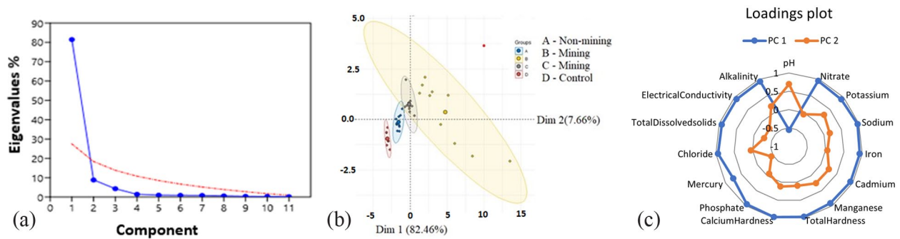
Figure 4. Principal component analysis of the metals and physicochemical parameters consisting of: (a) Scree plot, (b) 2D plot, and (c) Loadings plot.
