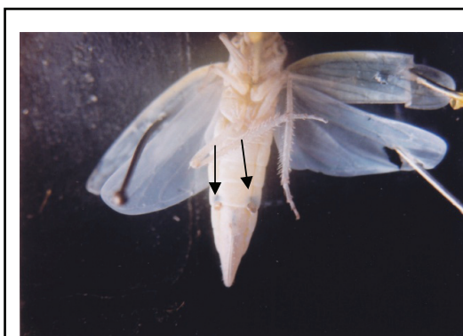
Plate 3. White leafhopper Cofana spectra styloped by Halictophagus australensis (Hyperparasitism indicated by arrow).
