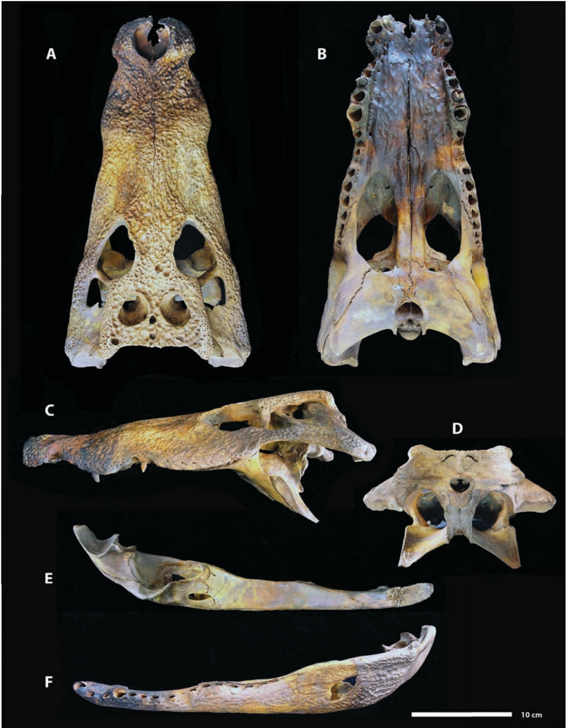
FIGURE 8. Skull and left mandible of a Cuban crocodile ( Crocodylus rhombifer ) of Late Quaternary age from Oleg's Bat Cave, Dominican Republic (MHD 574). Skull in A , dorsal, B , ventral, C , left lateral, and D , posterior views. Left mandible in E , medial and F , lateral views.
