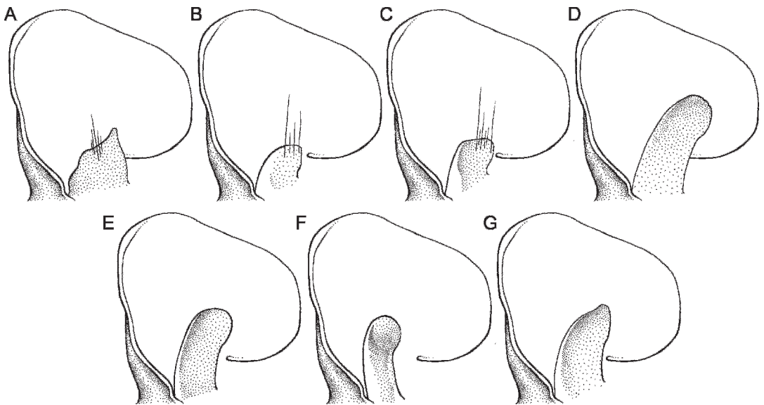
Fig. 4. Right ear and tragus of Miniopterus spp. from Madagascar: A , M. brachytragos (FMNH 175840, holotype), from Parc National de Namoroka, Forêt d'Ambovonombo, 26 km NW Andranomavo; B , M. brachytragos (FMNH 172685) from the Forêt de Binara, near Analamazava River, 7.5 km SW Daraina (village); C , M. brachytragos (FMNH 202523) from 1.8 km S Ambanizana, Masoala Peninsula; D , M. mahafaliensis (FMNH 173197, holotype) from Parc National de Tsimanampetsotsa, 6.5 km NE Efoetse, near Mitoho Cave; E , M. mahafaliensis (FMNH 176101) from Parc National de Kirindy-Mite, near village of Betakilotra, 11 km SE Marofihitsa; F , M. griveaudi (FMNH 184055) from Beloboka, grotte n°1, 12.5 km E Mahajanga, Madagascar; G , M. aelleni (FMNH 175842) from the Parc National de Namoroka, Forêt d'Ambovonombo, 26 km NW Andranomavo. The slightly elongated and pointed distal portion of the tragus in FMNH 175840 (A), as compared to FMNH 172685 and FMNH 202523, maybe an anomalous shape in M. brachytragos .
