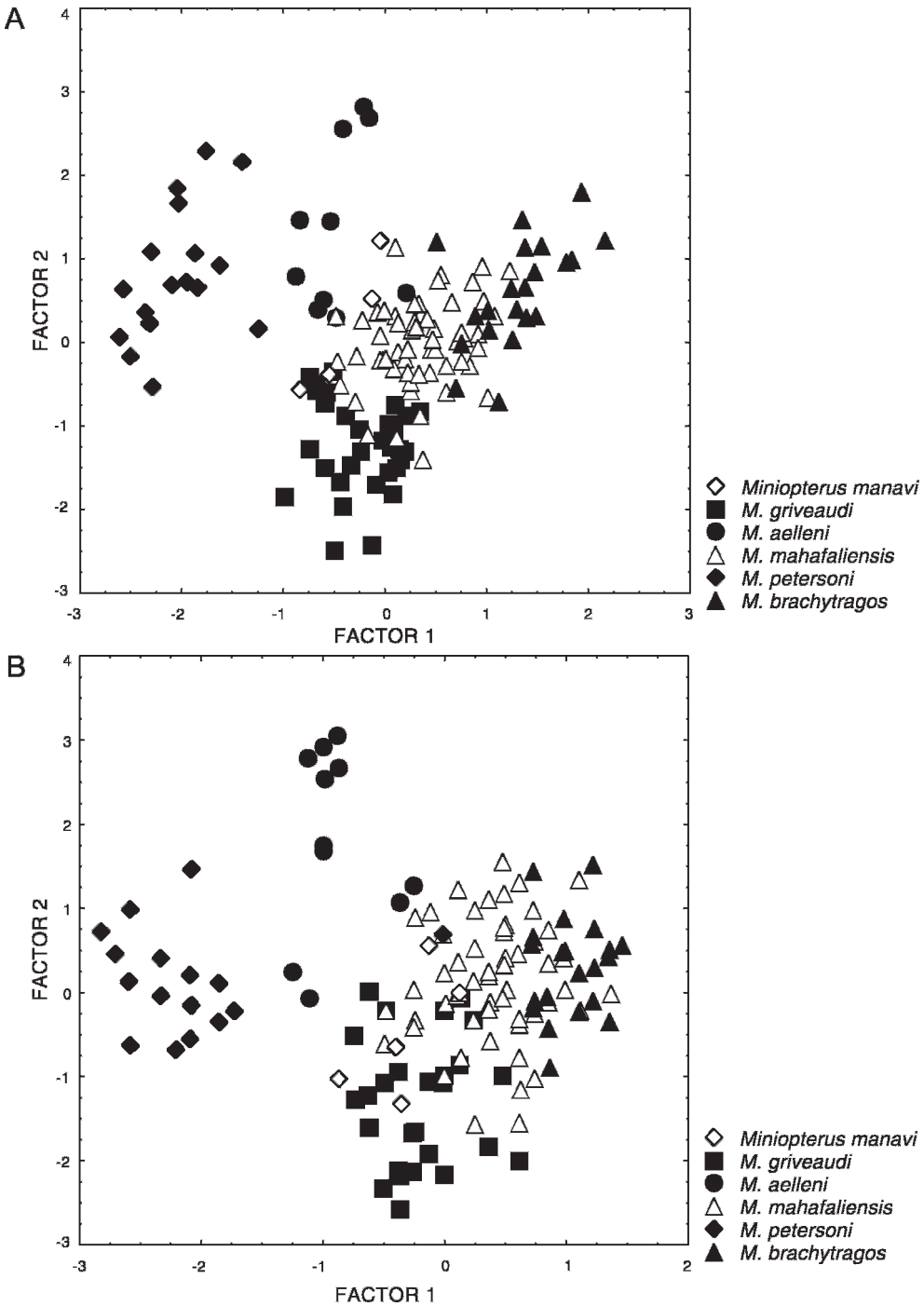
Fig. 11. Projections of factor 1 (x-axis) and factor 2 (y-axis) in principal component analysis of A , cranial measurements and B , dental measurements of different diminutive species of Miniapterus from Madagascar, all of which were previously considered to be M. manavi , as well as M. petersoni . Loadings of variables on each axis are shown in table 6.
