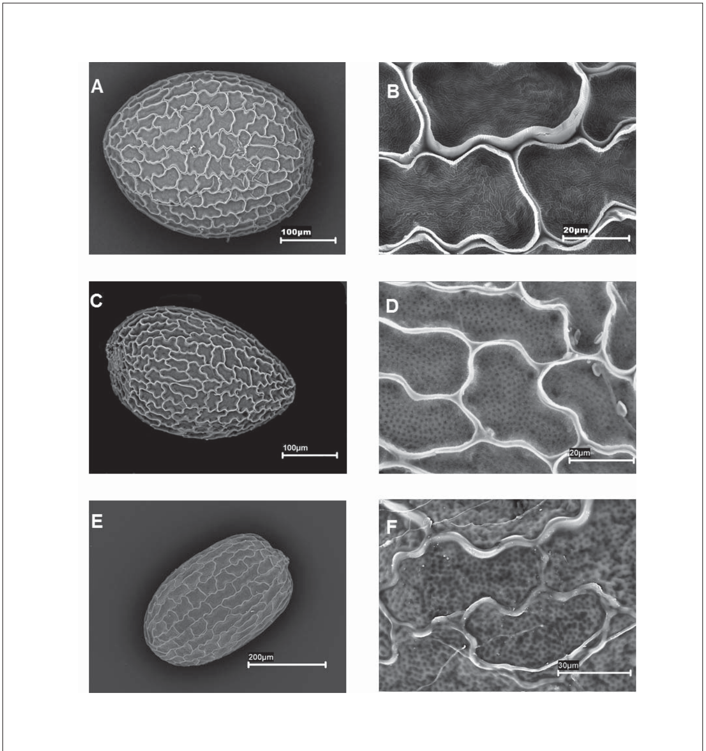
Fig. 2. – Seeds of different species of Erica L. A: Erica tetralix L.; B: E. tetralix (detail of surface cells); C: E. tetralix × E. ciliaris ; D: E. tetralix × E. ciliaris (detail of surface cells); E: E. ciliaris L.; F: E. ciliaris (detail of surface cells).
