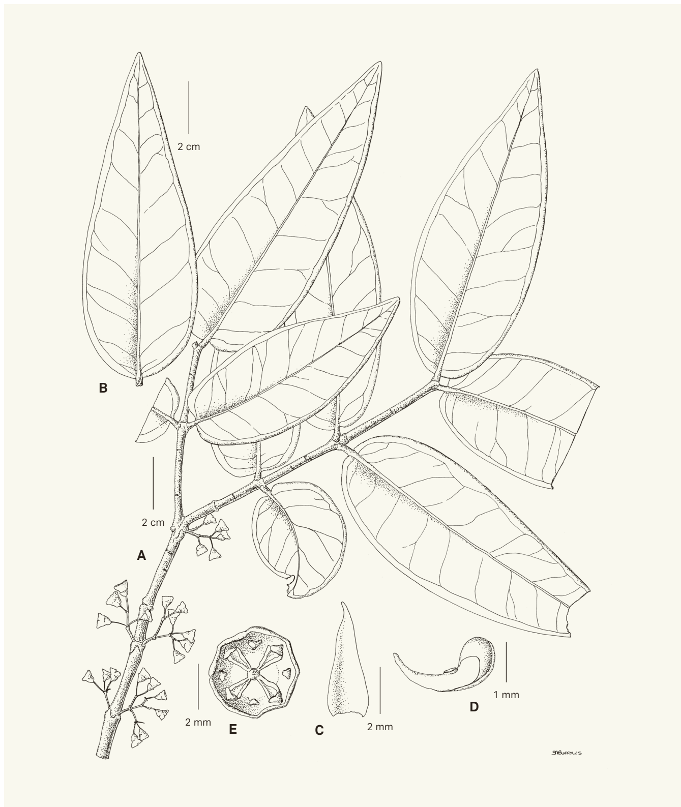
Fig. 10. – Memecylon unguiculare R.D. Stone. A. Flowering branch; B. Leaf; C. Petal; D. Anther; E. Epigynous chamber (top view). [Rabevohitra 2164, MO] [Drawing: S. Burrows]
