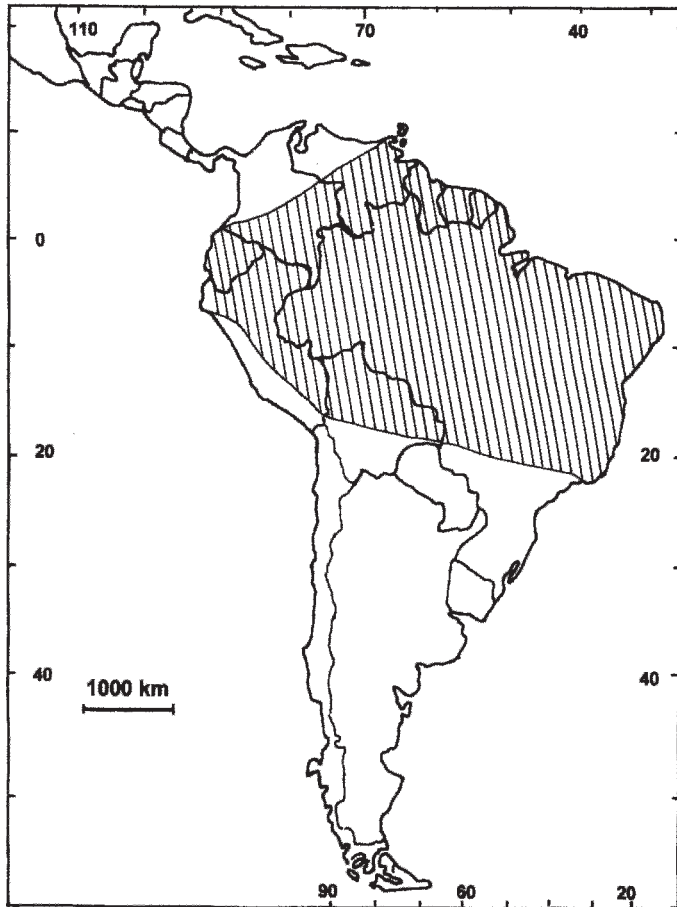
Fig. 3.—Geographic distribution of Choeroniscus minor .
