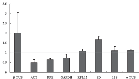
Fig. 5. The variation of expression of housekeeping genes in the whole bodies of Bactrocera dorsalis larvae under toxicity stress, and normalized by EF1 \alpha .
