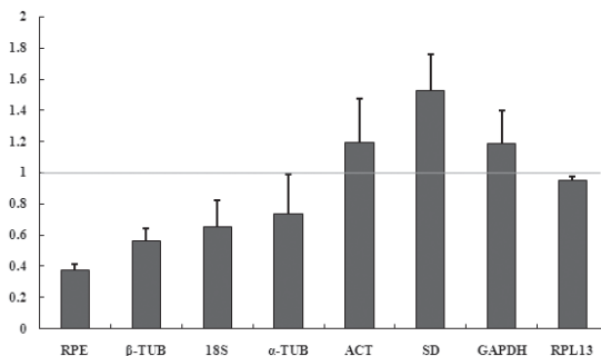
Fig. 6. The variation of expression of housekeeping genes in the midguts of Bactrocera dorsalis larvae under toxicity stress, and normalized by EF1 \alpha .
