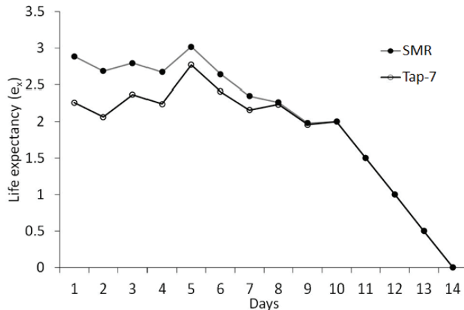
Fig. 4. Life expectancy of SMR and Tap-7 strains of Anastrepha ludens after aerial release.
