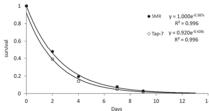
Fig. 3. Survival of SMR and Tap-7 strains of Anastrepha ludens after aerial release.
