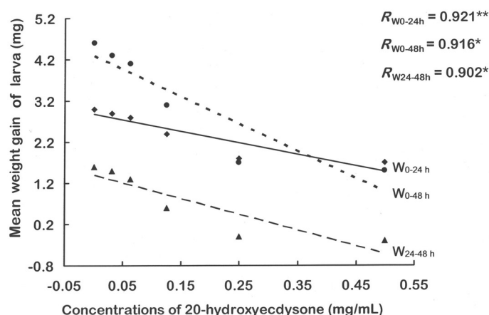
Fig. 4. The correlation between the concentration of 20-hydroxyecdysone in diet and mean weight gain in 4th instars of diamondback moth. W_{0-24h} , W_{0-48h} and W_{24-48h} represent mean weight gain at 24 h, at 48 h, and from 24 h to 48 h after treatment, respectively. R represents the coefficient; the symbols * and ** next to the coefficient indicate that the correlation between X and Y was significant at P < 0.05 and P < 0.01 , respectively.
