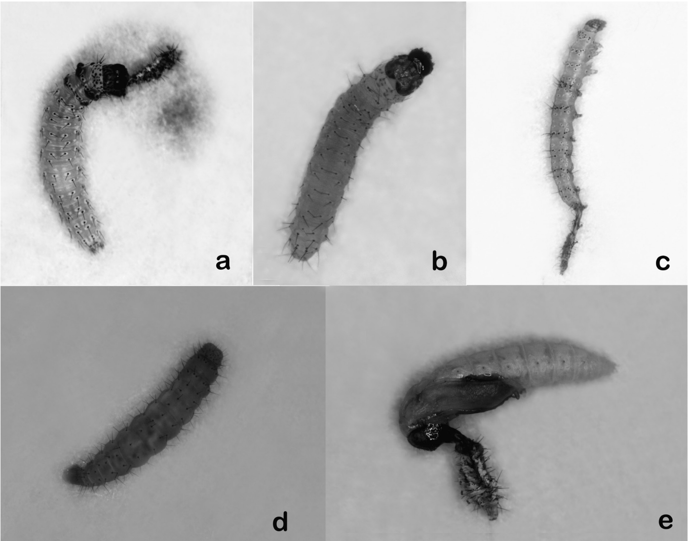
Fig. 6. The morphological changes in diamondback moth larvae and a pupae caused by ingestion of exogenous dietary 20-hydroxyecdysone. a, Exosmosis of ecdysial fluid and an additional molt (15 x); b, failure to shed the head capsule (30 x); c, failure to shed the exuvium (20x); d, bulging of the hindgut (10 x); and e, deformed pupa (10 x).
