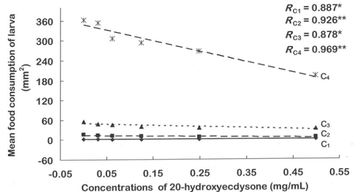
Fig. 2. The correlation between the concentration of 20-hydroxyecdysone in diet and mean food consumption by diamondback moth larvae for each instar. C_1 , C_2 , C_3 , and C_4 represent mean food consumption of 1st, 2nd, 3rd, and 4th instars, respectively. R represents the coefficient; the symbols * and ** next to the coefficient indicate that the correlation between X and Y was significant at P < 0.05 and P < 0.01 , respectively.
