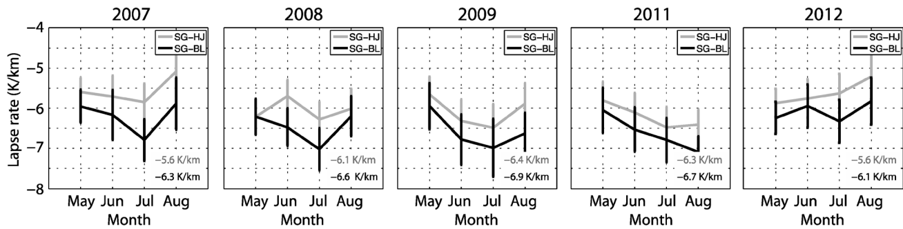
FIGURE 6. Mean monthly lapse rates between South Glacier AWS (SG) and valley stations Burwash Landing (BL) and Haines Junction (HJ) calculated for melting conditions ( T > 0\text{ }^{\circ}\text{C} ) at SG. Mean values for the model calibration period are listed for each year.
