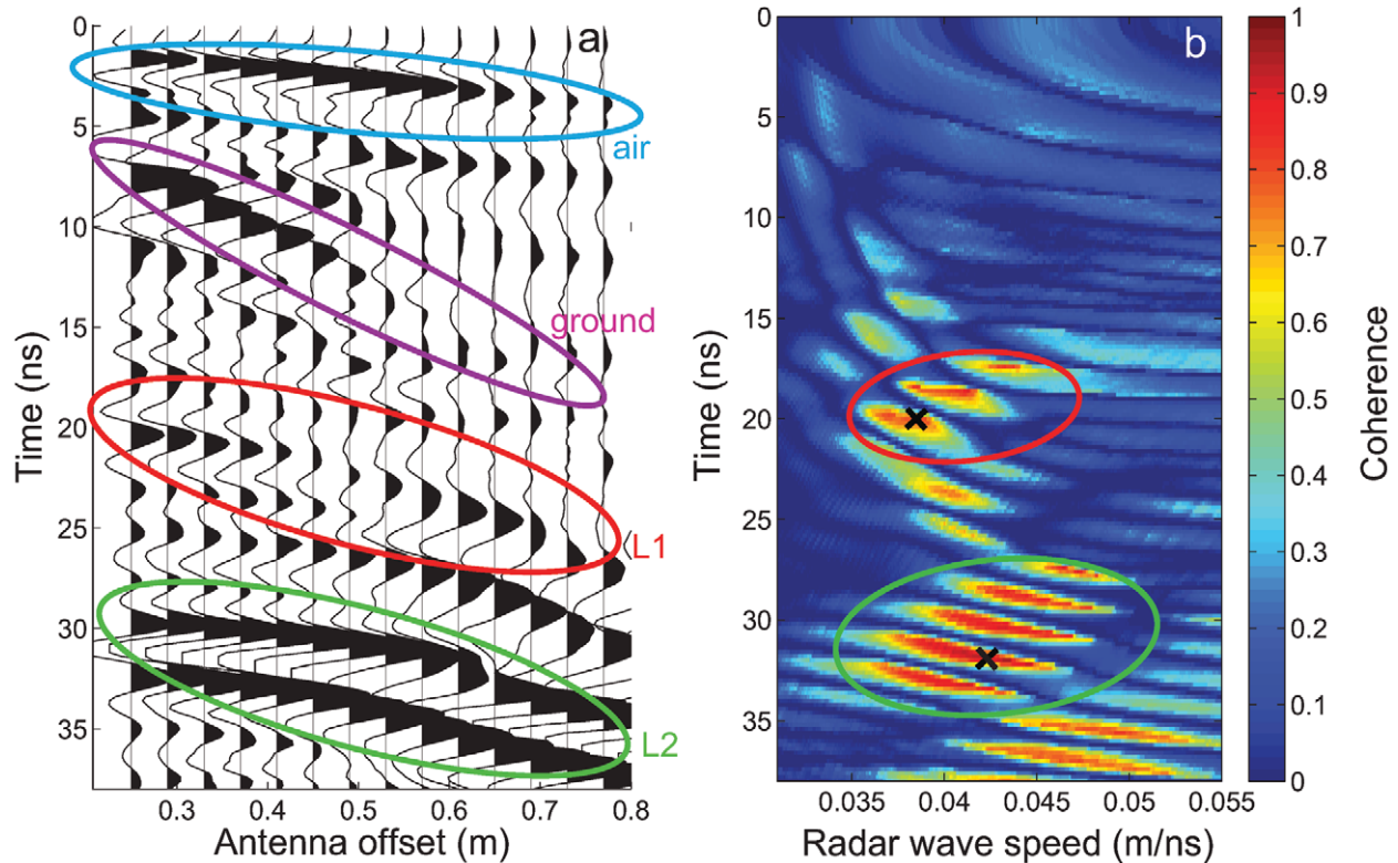
FIGURE 2. (a) The 500 MHz Common Mid Point gather and (b) coherence plot at our study site. The CMP gather (a) shows two coherent hyperbolic reflections: L1 (red) corresponds to the transition from peat to silt and L2 (green) corresponds to the permafrost table. Peaks in the coherence plot (crosses in b), allow normal-move-out velocity determination (Equation 1).
