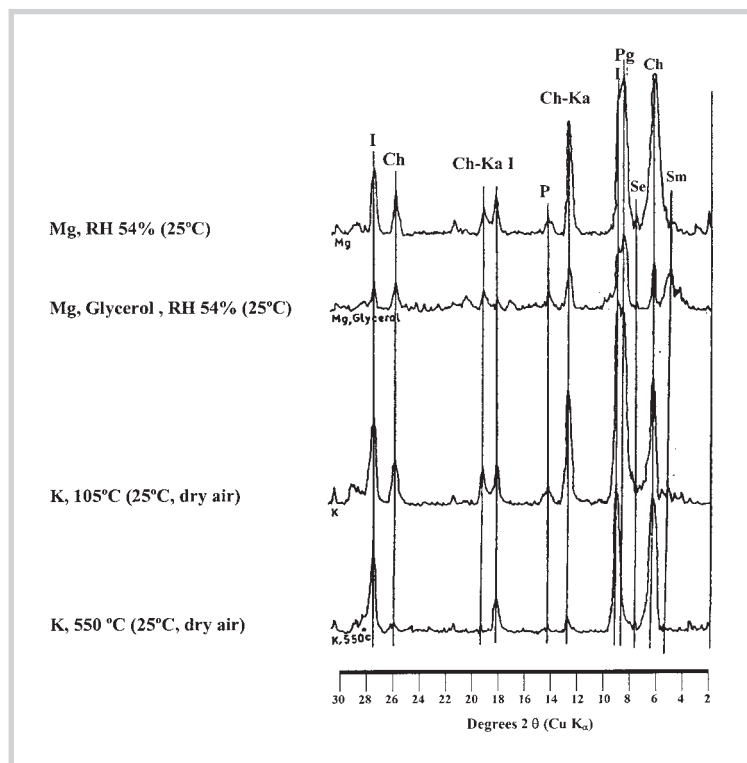
FIGURE 2 XRD patterns for the <2- \mu\text{m} fraction of the treated alluvium from the BZ1. I: Illite; Ch: Chlorite; P: Plagioclase; Pg: Palygorskite; Se: Sepiolite; Sm: Smentite; RH: relative humidity. (XRD patterns prepared by A. Yathrebi)
