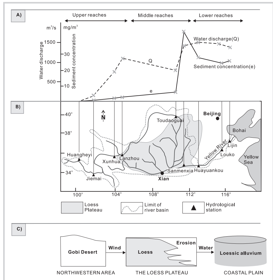
FIGURE 2 Natural scenario of the Loess Plateau and the Yellow River: (A) large increase in water discharge ( \text{m}^3/\text{s} ) and sediment concentration ( \text{mg}/\text{m}^3 ) in the Yellow River after it runs through the Loess Plateau (after Ren and Zhu 1994); (B) geographical location of the Loess Plateau and the Yellow River (after Xu 1999); (C) geological relations between the Gobi Desert in the northwest, the central Loess Plateau, and the eastern coastal plain (after Rutter 1992; Derbyshire and Wang 1994).
