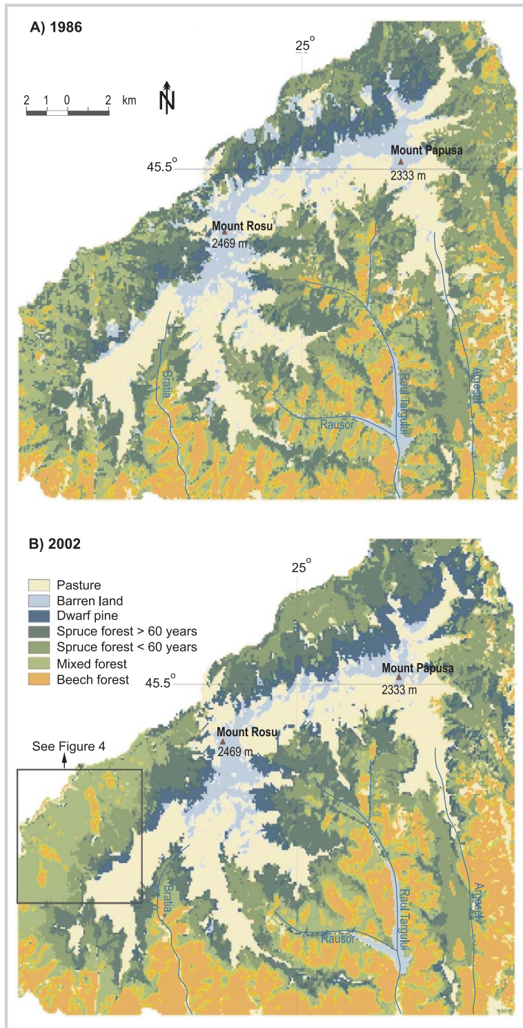
FIGURES 2A AND 2B Altitudinal zones of vegetation in the Iezer Mountains in 1986 (A) and 2002 (B).
