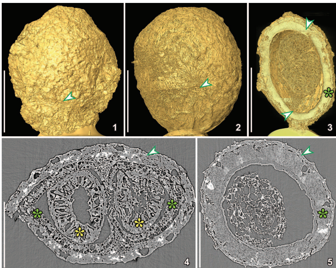
FIGURE 6—Three-dimensional (1–3) and 2-D (4, 5) SRXTM reconstructions of two charcoalfied fruits with similar external morphology, but different internal structure; 1, surface rendering of Canrightia resinifera (S171508) from the Early Cretaceous Catefica locality, Portugal, showing slightly wrinkled surface of fleshy fruit wall and short hypanthium (arrowhead); dataset acquired using 10 \times objective and a 20 \mu m thick LAG:Ce scintillator at 10 keV (voxel size 0.74 \mu m); 2, surface rendering of Canrightia -like fruit (S174033) from the Early Cretaceous Famalicão locality, Portugal, showing slightly wrinkled surface of fleshy fruit wall and scars from stamens (arrowhead) on the fruit surface; dataset acquired using 20 \times objective and a 20 \mu m thick LAG:Ce scintillator at 10 keV (voxel size 0.325 \mu m); 3, combined surface rendering and cut voltex (transparent rendering) of Canrightia -like fruit (S174105) from the Early Cretaceous Buarcos locality, Portugal, in longitudinal section showing a single, hemi-orthotropous and pendulous seed with chalaza and vascular bundles entering the seed close to apex (arrowhead) and micropyle directed towards the base (arrowhead) and with thick crystalliferous endotesta (green asterisk); dataset acquired using 20 \times objective and a 20 \mu m thick LAG:Ce scintillator at 10 keV (voxel size 0.325 \mu m); 4, transverse orthoslice of Canrightia resinifera (same dataset as for 1) showing fruit wall (arrowhead) enclosing two ovules/seeds with the seed wall composed of crystalliferous and fibrous endotesta (green asterisks) and a thick endotegmen composed mainly of endothelium cells (yellow asterisks); 5, transverse orthoslice of Canrightia -like fruit with collapsed fruit wall (arrowhead) enclosing a single seed (same dataset as for 2); seed wall mainly composed of crystalliferous and fibrous endotesta and with grooves giving the seed surface a pitted appearance; inside are remains of endosperm and embryo. Scale bars for 1–3=500 \mu m; for 4, 5=250 \mu m.
