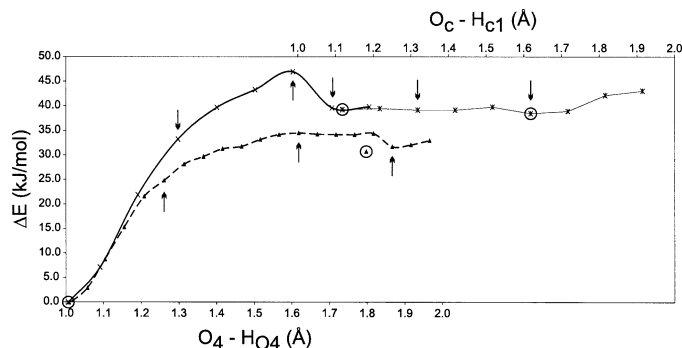
FIG. 4. Energy change upon elongation of the O_4-H_{O_4} bond in the \langle a2bc \rangle ( \blacktriangle ) and \langle a3bc \rangle ( \times ) model space and upon further elongation of the O_c-H_{c1} bond in \langle a3bc \rangle (*). The energy of the PrimCat + species is taken as reference (respectively -555.686 and -833.520 atomic units). Optimized points are indicated by circles, arrows point out proton transfers.
