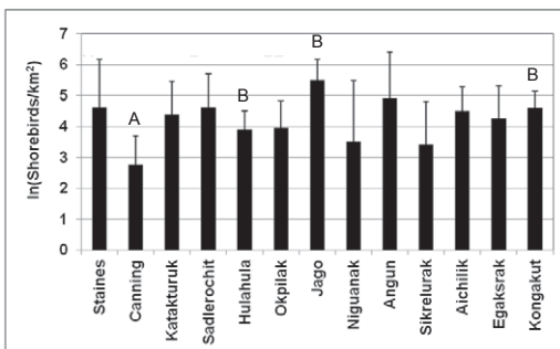
Figure 2. ln(density estimates) and associated 95% confidence intervals for river deltas on the coast of the Arctic National Wildlife Refuge, Alaska, from surveys conducted between 2006 and 2010. Deltas with different letters had significantly different density estimates in the Tukey-Kramer multiple comparisons test.
