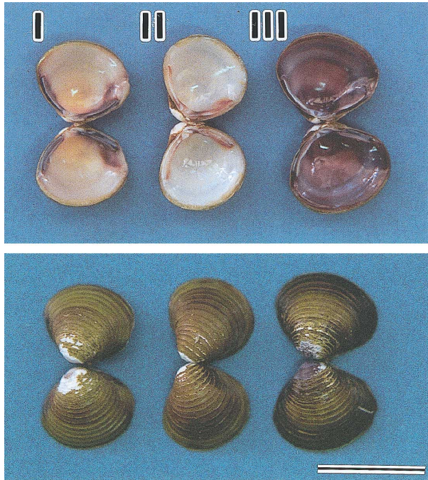
Fig. 1. External and internal views of the three type of Corbicula fluminea collected in Hou Don, Taiwan. (Left; type I, middle; type II, right; type III) Scale: 10 mm.
