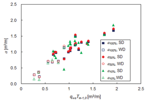
Figure 7. The Weibull scale parameter a versus overtopping parameter q_{ws}T_{m-1,0} .
