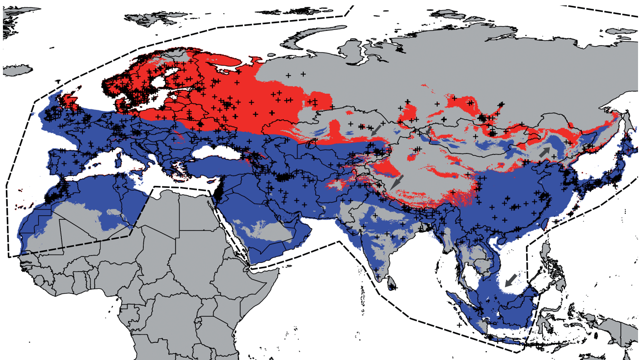
Fig. 3. Present-day and Last Glacial Maximum projections of ecological niche models for great tits ( Parus major sensu lato ) across Eurasia and North Africa. Dashed black line indicates the limits of the hypothesis of M used in model calibration. Black crosses indicate known occurrences of the species under present-day conditions. Red area shows present-day potential distribution (note that this area is partly obscured by the blue areas); blue area shows model transfer to Last Glacial Maximum conditions, as summarized by the MIROC general circulation model simulation. Arrows represent points of reference for discussion in text.
