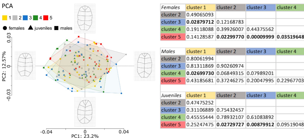
Fig. 4. Differences in plastron shape among genetic clusters determined by DAPC. The ordination plot shows the first two PCA components describing the variability in the shape of the plastron. The table shows significance values for the test of differences in plastron shape for individual clusters.
