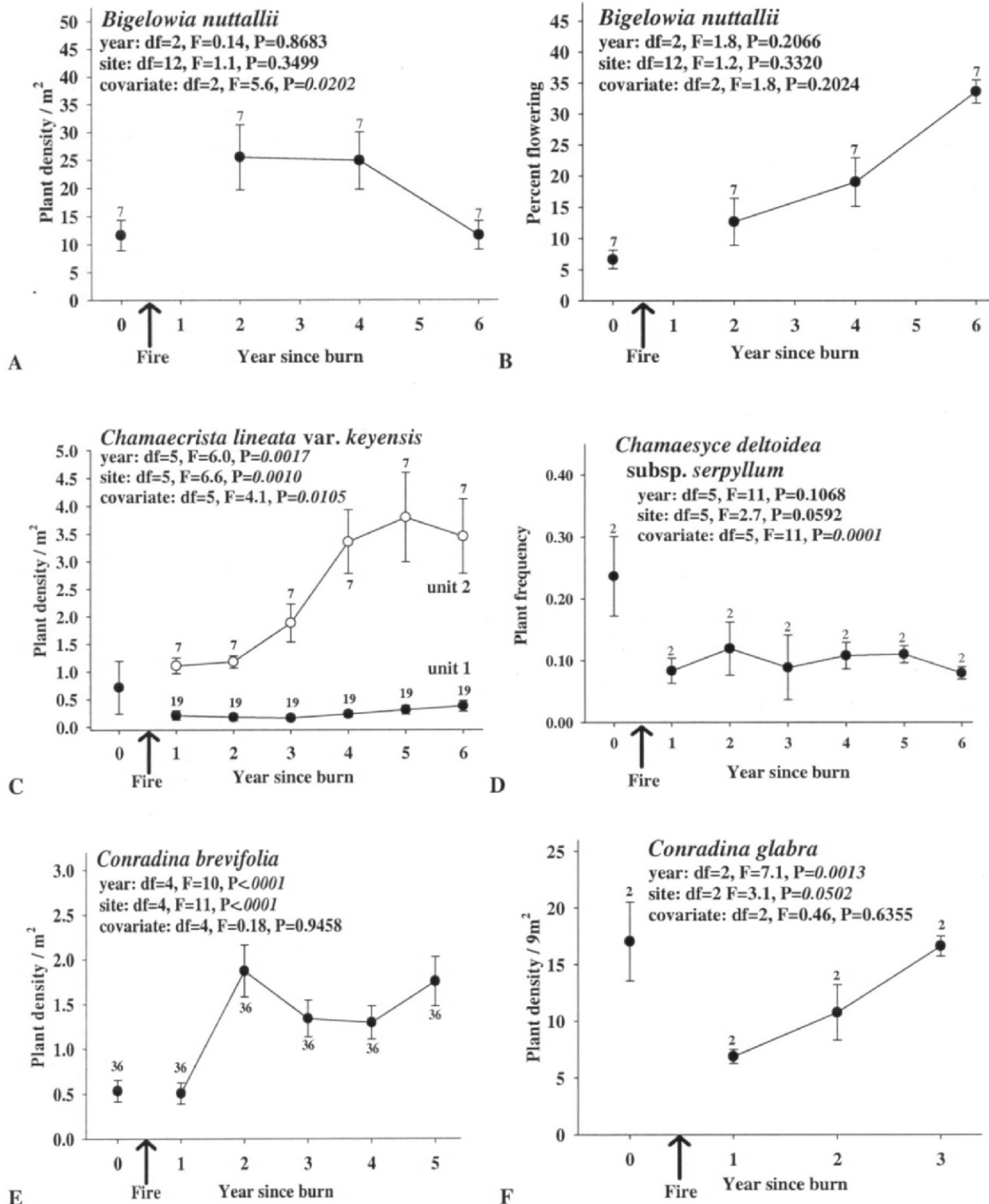
Figure 2. Species whose variables (A through F) were analyzed with repeated measures analysis of covariance ( P < 0.05 ). The value separated from the line at 0 year since burn represents the covariate value: the pre-burn or long-unburned population condition. All graphs shown are \pm 1 SE. Number above or below error bar denotes sample size. Where mean change obscures significant trends, population responses are shown separately. Significant p-values are italicized. Variable A = Bigelowia nuttallii density, B = B. nuttallii percent flowering, C = Chamaecrista lineata var. keyensis density, D = Chamaesyce deltoidea subsp. serpyllum frequency, E = Conradina brevifolia density, F = C. glabra density.
