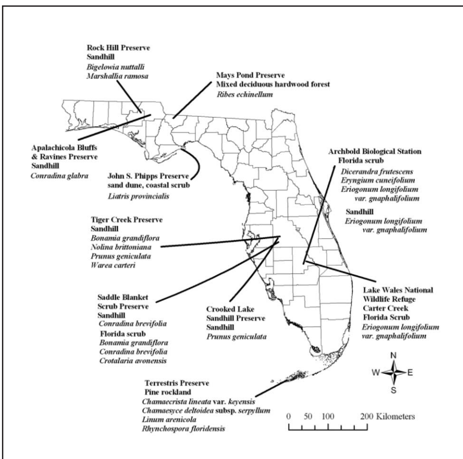
Figure 1. Ten preserves, their associated habitat(s) and 18 species monitored in Florida.
