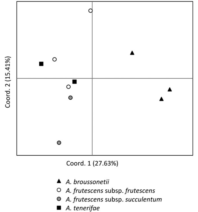
Fig. 4. Principal coordinates analysis (PCoA) of 10 samples of Argyranthemum based on genotypic information from eight SSR loci.
