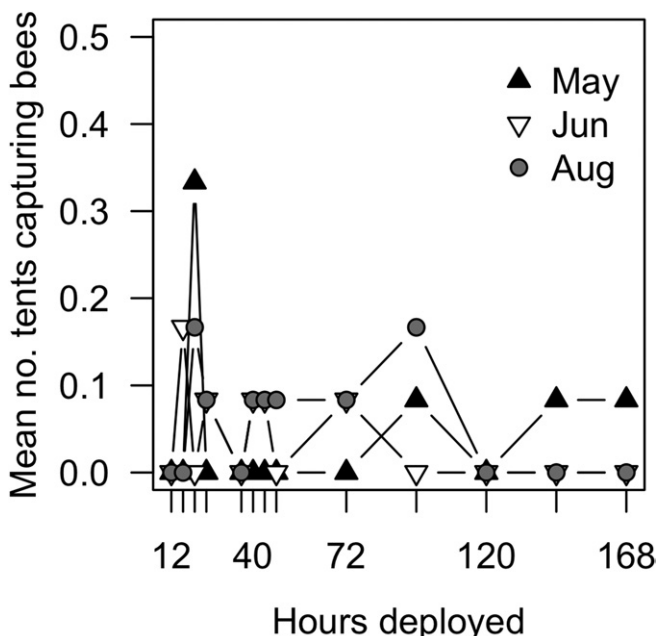
Fig. 1. Proportion of tents capturing bees over time by month at Site 2.
