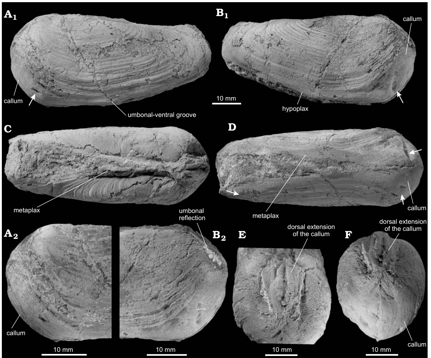
Fig. 5. Pholadidea gradzinskii sp. nov. (ZPAL Mo. XVIII/3, holotype) from the Oligocene of King George Island. A. Left-lateral view of the complete specimen (A 1 ), arrow marks deformation of the callum; anterior of the left valve (A 2 ), showing callum covered with growth lines. B. Right-lateral view of the complete specimen (B 1 ), arrow marks deformation of the callum; anterior of the right valve (B 2 ), showing umbonal reflection raised anteriorly and appressed on the umbo. C. Dorsal view of the complete specimen showing metaplex formed by partially calcified periostracal mantle connecting the dorsal margin of the valves. D. Ventral view of the complete specimen showing a hypoplax formed by partially calcified periostracal mantle extending beyond the ventral margin of the shells and connected with the callum; arrows mark deformation of the callum and hypoplax. E. Inclined dorsal view of the anterior showing umbonal reflection covered with the dorsal extension of the callum. F. Anterior view showing the callum and umbonal reflection covered by the dorsal extension of the callum.
