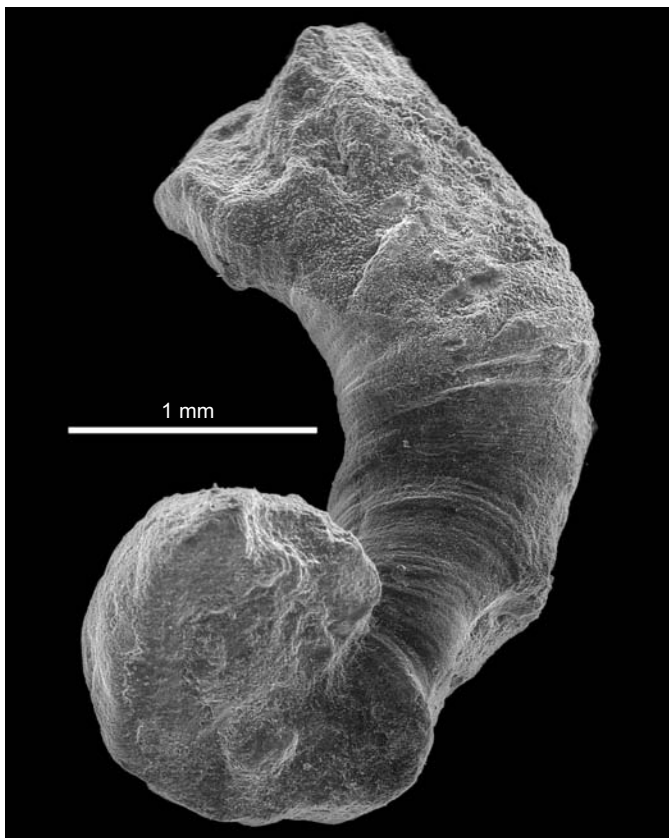
Fig. 2. Isolated origin of microconchid tubeworm Helicoconchus elongatus gen. et sp. nov. (scanning electron micrograph), NHM PI AN 1184.
