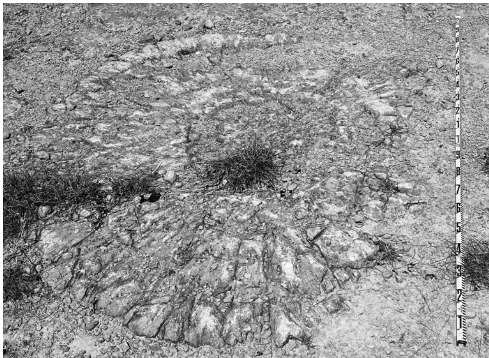
Fig. 3. Microconchid tubeworm Helicoconchus elongatus gen. et sp. nov. reef in the lower portion of the E unit of the Bead Mountain Formation (Lellis and Holterhoff, 2010) and more specifically the 3B cycle set of Lellis (2010) at location N latitude 32° 41' 39.31", W longitude 99° 22' 58.37". Viewed from above. The radiating surficial pattern is due to weathering. The scale is numbered in tenths of meters. Photograph courtesy of Peter Holterhoff.
