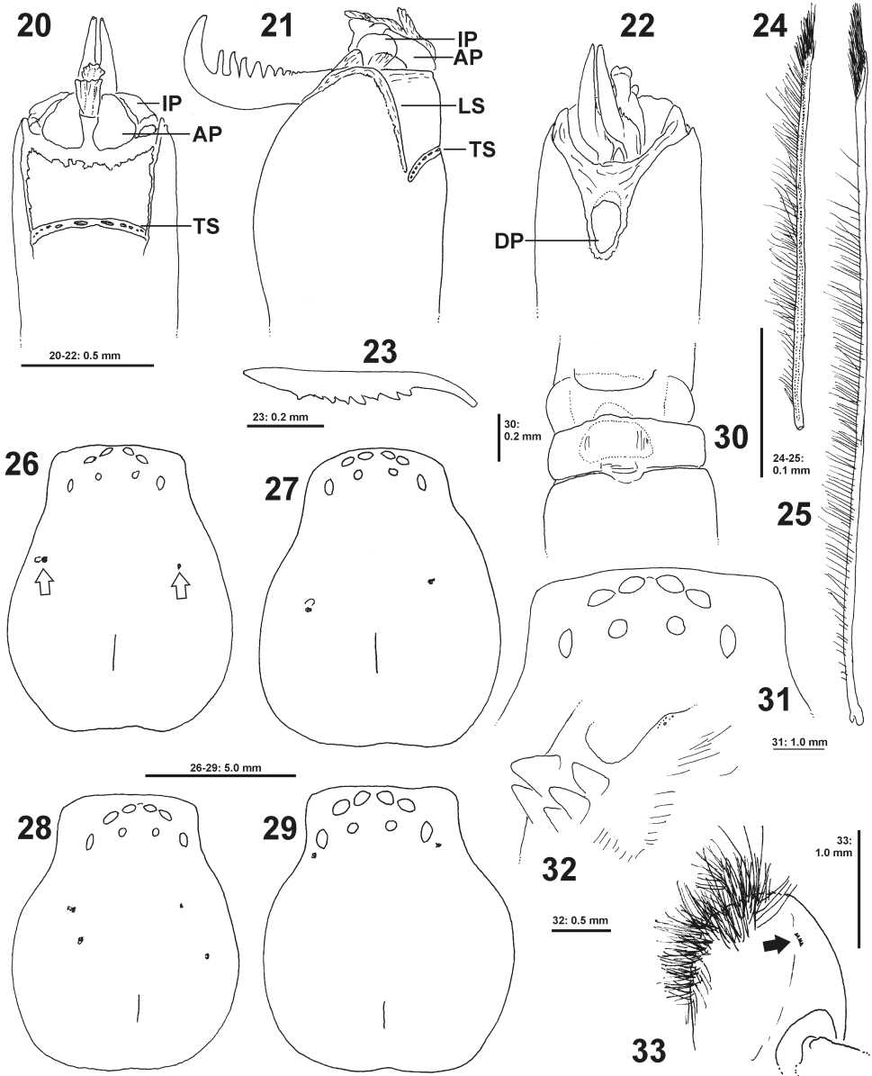
Figs 20–33. May bruno gen. n. sp. n. from South Africa (♀ paratypes from Witsand, ♀ from Twee Rivieren): (20–22) tarsus tip: (20) ventral, (21) lateral, (22) dorsal; (23) ♀ palpal claw, lateral; (24–25) Lawrence setae; (26–29) prosoma of ♀♀, showing positions of dorsal marks (white arrows in Fig. 26); (30) metatarsal stopper, dorsal; (31) eye arrangement, dorsal; (32) cheliceral dentition, ventral; (33) gnathocoxae, ventro-distal, showing reduced serrula (black arrow). Abbreviations: AP – plate of Lawrence setae; DP – dorsal plate of elongated setae; IP – plate of indented claw tuft setae; TS – transverse suture with slit sensilla.
