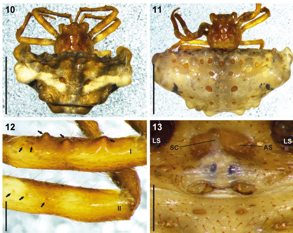
Figs 10–13. Digital microscope photographs of Pasilobus dippenaarae sp. n.: (10) habitus of holotype; (11) same, paratype; (12) dorso-prolateral view of femora I and II, arrows indicating large and small tubercles; (13) paratype, ventral epigyne. Abbreviations: AS – anterior sclerite; LS – lateral sclerite; SC – scape. Scale bars: (10, 11) = 5 mm; (12, 13) = 0.5 mm.
