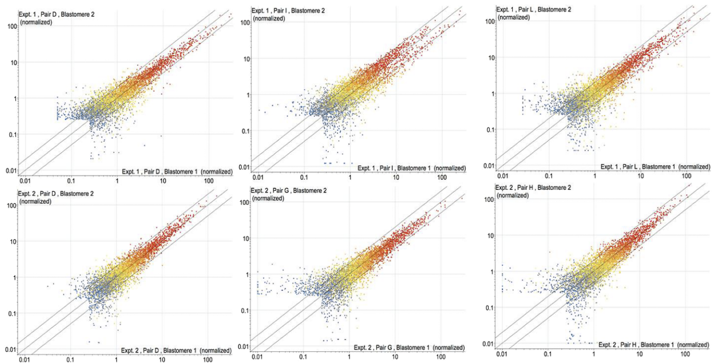
FIG. 2. Scatter plot analysis across blastomere pairs. Genes present above background level and with normalized expression values >0.25 in at least one blastomere from all pairs (4573 genes) are displayed normalized to the 75th percentile of the array and further scaled assuming maximum correlation for all genes within and across pairs. Diagonal lines indicate 2-fold differential expression. Red = high expression; yellow = median expression; blue = low expression.
