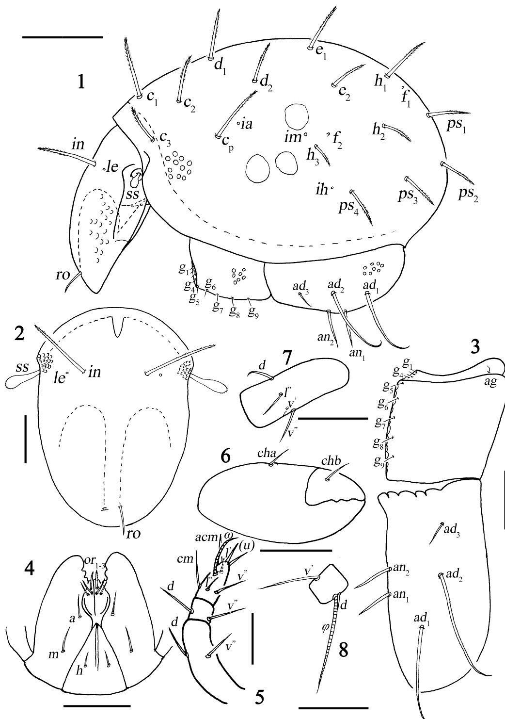
FIGURES 1–8. Notophthiracarus motumuka sp. nov.: 1, lateral view of body (legs removed); 2, prodorsum, dorsal view; 3, left side of ventral plate; 4, subcapitulum, palpi removed; 5, palp, antiaxial view; 6, chelicera, antiaxial view; 7, femur I; 8, tibia IV. Scale bars: 1=100µm; 2–4, 6–8=50µm; 5=25µm.
