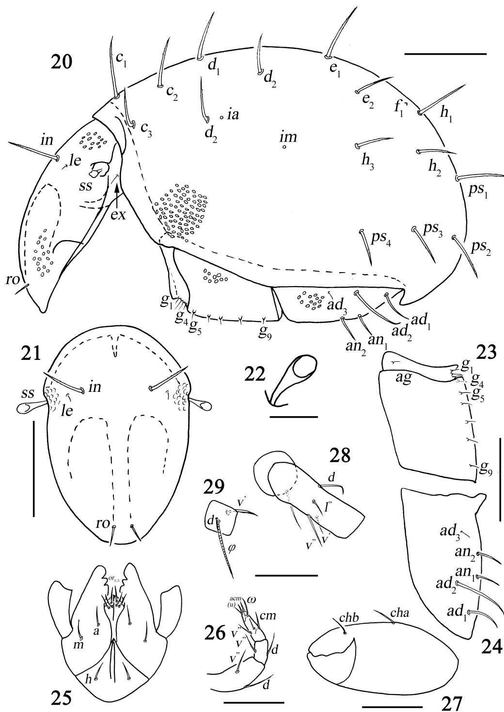
FIGURES 20–29. Notophtiracarus rimi sp. nov.: 20, lateral view of body (legs removed); 21, prodorsum, dorsal view; 22, sensillus, dorsal view; 23, right side of genito-aggenital plate; 24, right side of ano-adanal plate; 25, subcapitulum, palpi removed; 26, palp, antiaxial view; 27, chelicera, antiaxial view; 28, trochanter and femur I; 29, tibia IV. Scale bars: 20–21, 23–24=100µm; 25–29=50µm; 22=25µm.
