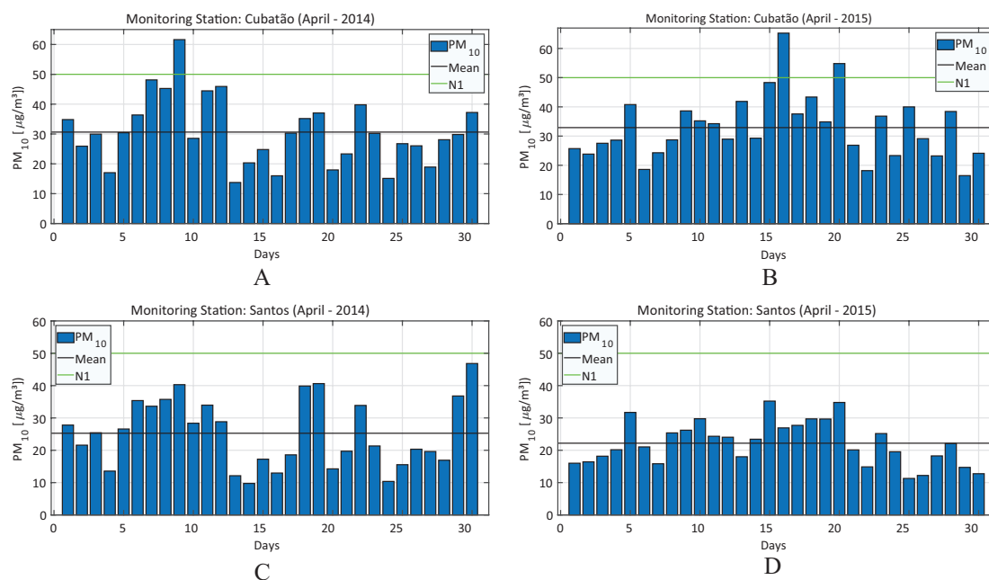
Figure 6. Graphs of PM 10 emissions monitored at Cubatão and Santos in 2014 and 2015. Figure A corresponds to the PM10 values at the Cubatão station during April 2014. Figure B corresponds to the PM10 values at the Cubatão station during April 2015. Figure C corresponds to the PM10 values at the Santos station during April 2014. Figure D corresponds to the PM10 values at the Santos station during April 2015.
