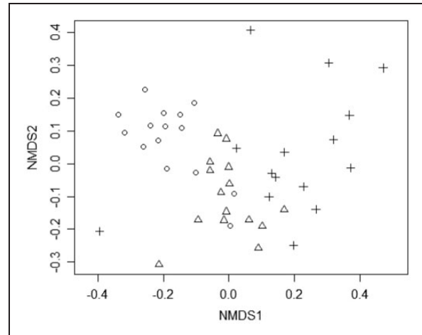
Figure 2. Floristic groups corresponding to the altitudinal level in the mountain of Bodocongó in the semiarid region of Brazil. The samples (plots) are ordered for each of the two dimensions of a nonmetric multidimensional ordination performed using site abundance-based Bray–Curtis similarity matrix and altitude (see Method section for details). Circles are the L1 plots, triangles are the L2 plots, and crosses are the L3 plots.
