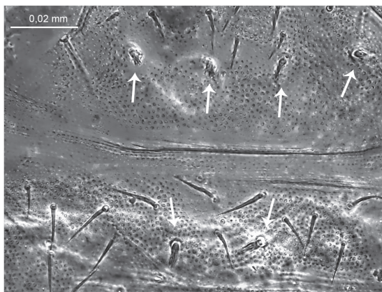
Figs. 27–32. Protaphorura salsa sp. nov. : (27) AIIIO; (28) PAO; (29) Furcal area; (30) Abd. sterna II and III with mvo, preadult male; Protaphorura bakhchisaraica sp. nov. : (31) Abd. sterna II and III with mvo, adult male; P. stiriaca (Stach, 1946): (32) Abd. sterna II and III with mvo, adult male. Arrows show the modified chaetae.
