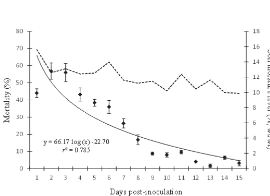
Fig. 2. Mortality of Anastrepha ludens larvae caused by Heterorhabditis bacteriophora IJs in a sandy clay soil undergoing the loss of moisture. The bars represent the standard error of mean mortality. (—) Represents larval mortality and (----) represents the soil moisture level.
