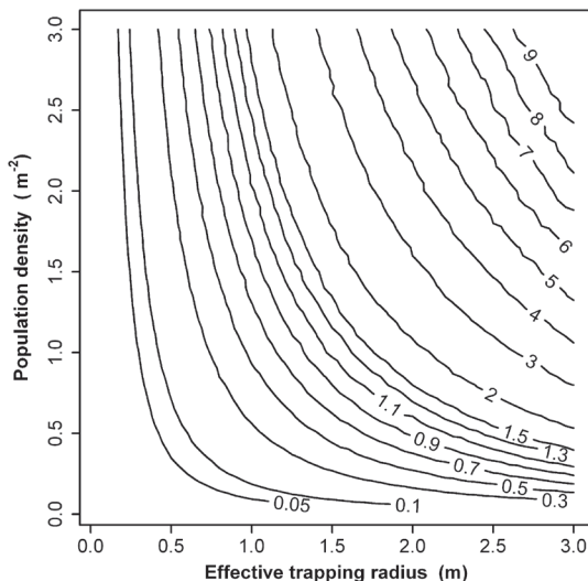
Fig. 4. Contours of the standard errors of the residuals between the simulated and TCM-estimated densities at various effective trapping radii. The distance classes ranged from 0 to 3 m at an interval of 1 m, with 5,000 replications for simulated paired traps per distance class. The coefficient of variation (CV) in density was assumed to be 10%.
